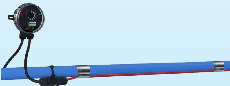
Example of assembly on one heat tracing cable, with Y24 connection box, for PVC pipe antifreeze protection
